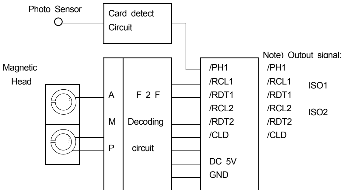
Fig 7.1 Block diagram
